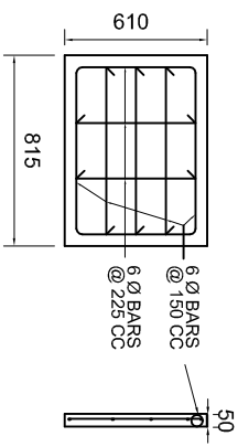
DETAIL 'D' R.C.C. SLAB AS CURB
