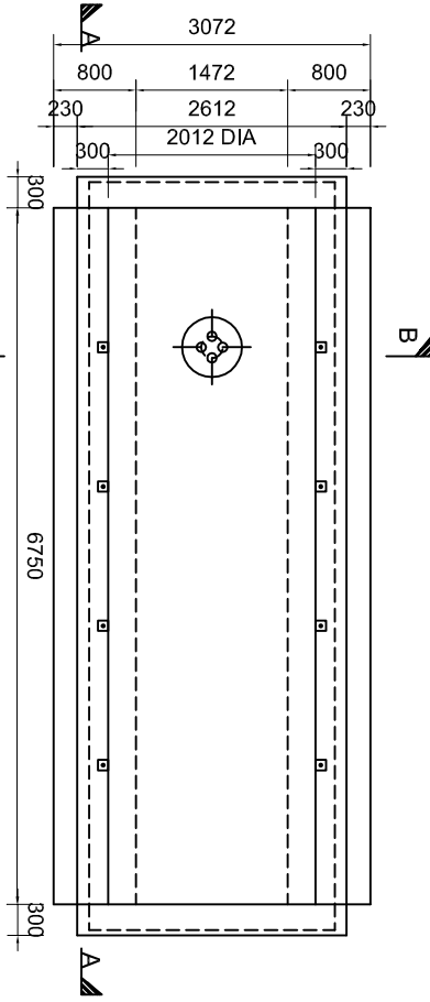
PLAN
